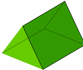
Triangular prism
