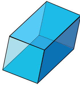
Cuboid
