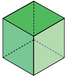
Cube
