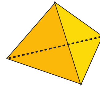
Tetrahedron
